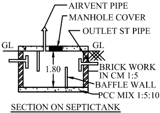
SECTION ON SEPTICTANK
