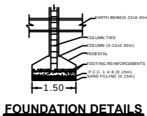
FOUNDATION DETAILS
