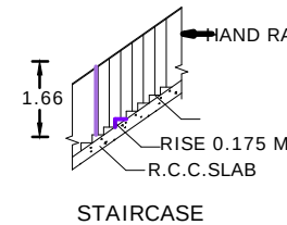
STAIRCASE
