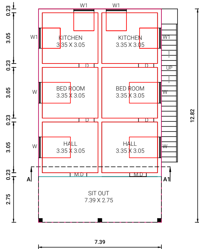
PLAN - GROUND FLOOR (PROPOSED)
