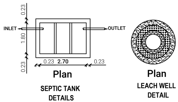
SEPTIC TANK DETAILS
