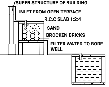
DETAILS OF FILTER BED & WELL
