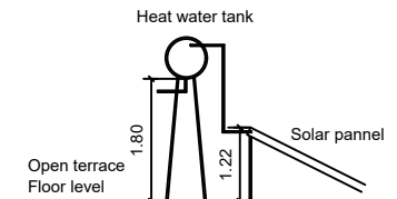
SIDE ELEVATION
