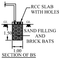
SECTION OF BS
