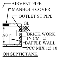
ON SEPTICTANK
