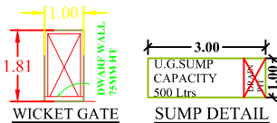
WICKET GATE
