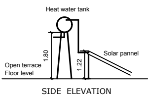
SIDE ELEVATION
