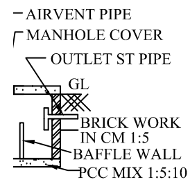
SEPTICTANK
