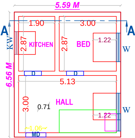
PLAN - GROUND FLOOR (PROPOSED)
