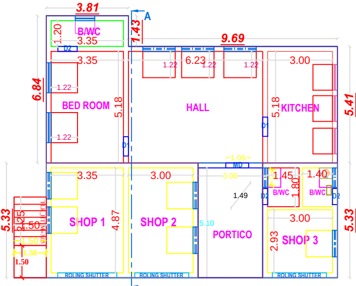
PLAN - GROUND FLOOR
