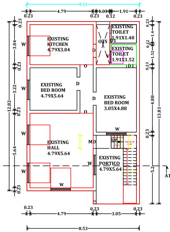
E GROUND FLOOR
