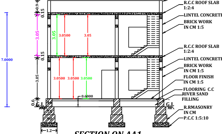
SECTION ON AA1
