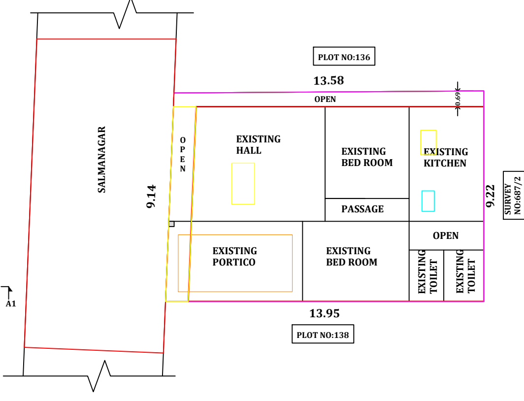
SITE PLAN
