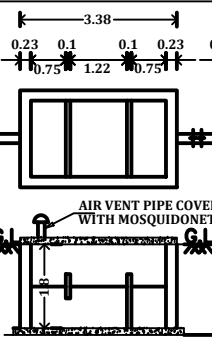
PLAN & SECTION OF SEPTIC TANK 'U' TRAP PROVIDED
