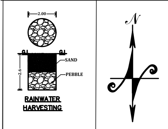
DETAILS SCALE 1:50
