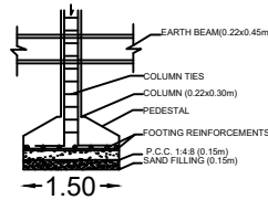
FOUNDATION DETAILS
