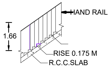
STAIRCASE
