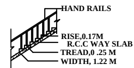
SECTION ON STAIR
