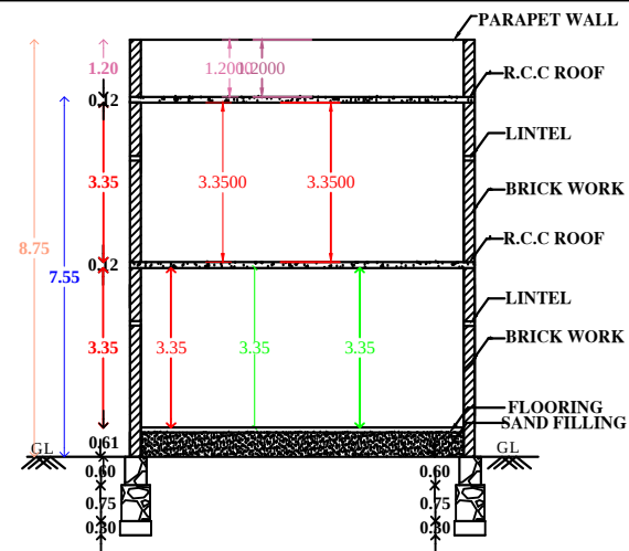
"SECTION "AB"
