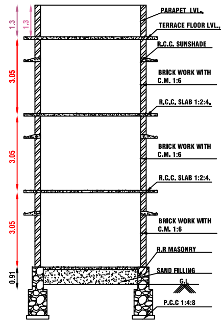
SECTION ON A-A' & B
