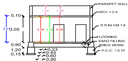
SECTION AB
