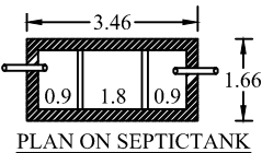
PLAN ON SEPTICTANK
