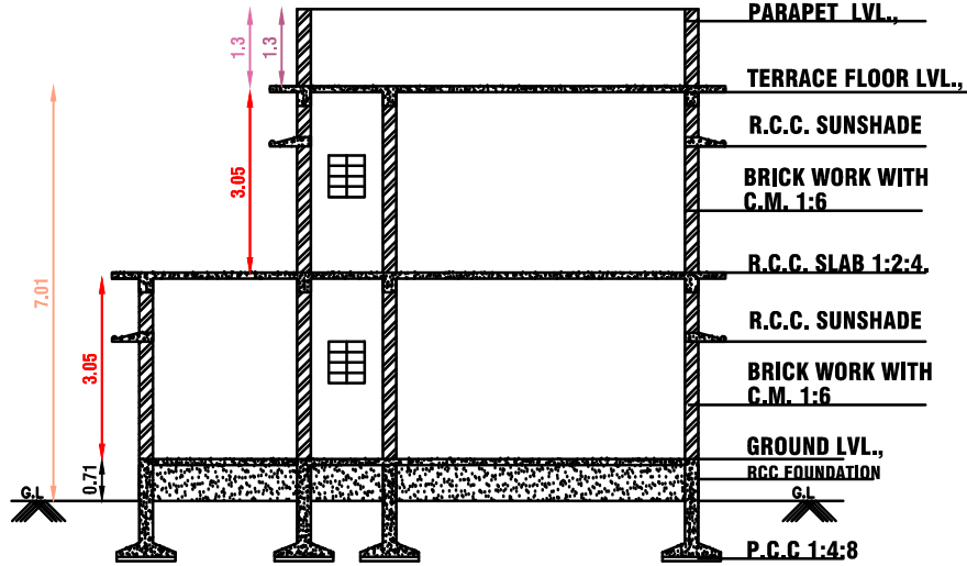
SECTION ON A-A & A'-A'
