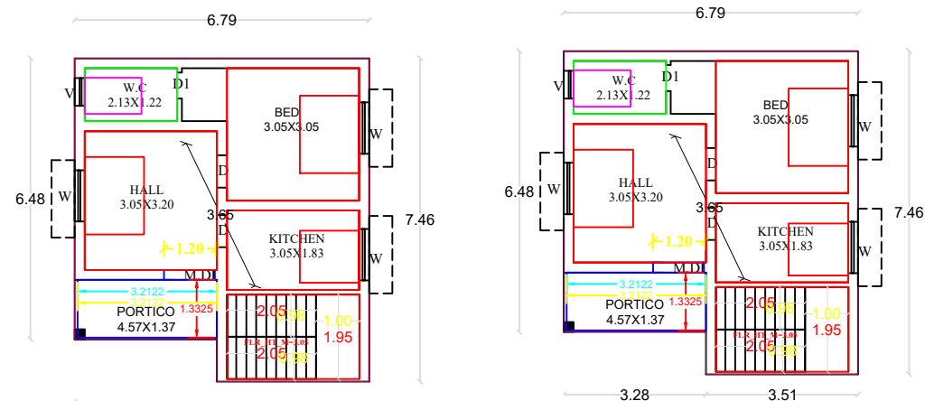
BLOCK -2 GROUND FLOOR PLAN
