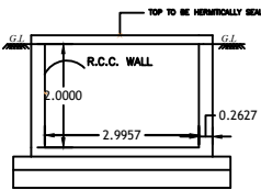
RWH SECTION
