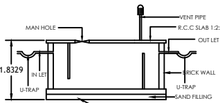
SECTION E.F. SEPTIC TANK
