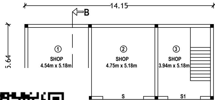
PLAN (BASEMENT FLOOR)
