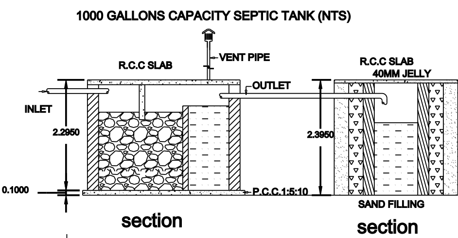
section
