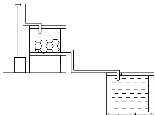
DETAILS OF FILTER BED & WELL
