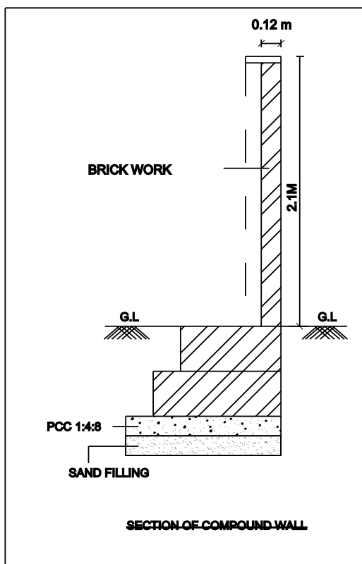
SECTION OF COMPOUND WALL
