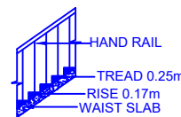
STAIR CASE DETAIL
