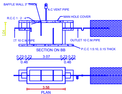
EPTIC TANK AND TRENCH & U TRAP ADOPTED
