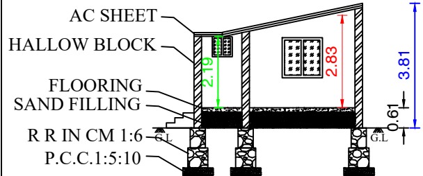
SECTION AB
