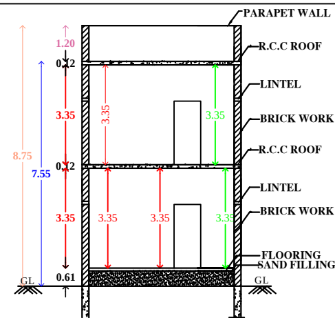
"SECTION "AB"
