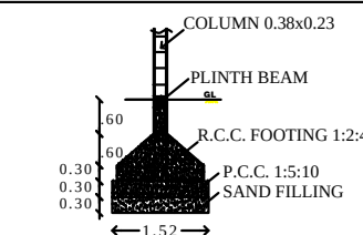
COLUMN DETAILS
