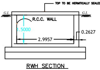
RWH SECTION
