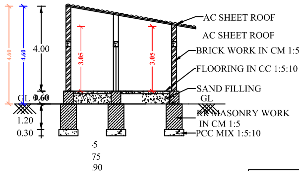
SECTION ON "BS"
