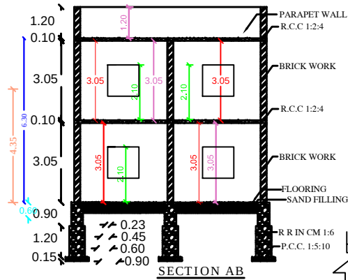
SECTION AB
