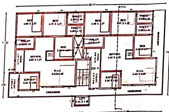
FLOOR 2 PLAN
