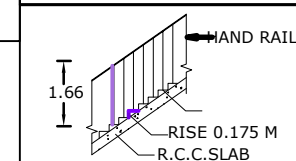
STAIRCASE
