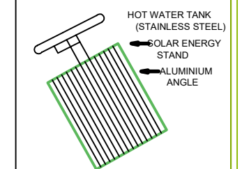
DETAILS OF SOLAR WATER HEATER
