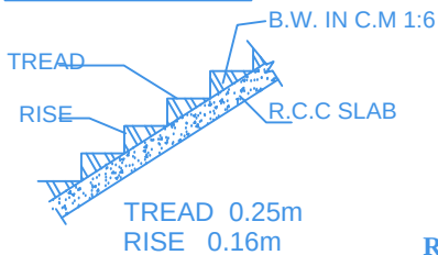
STAIR DETAILS
