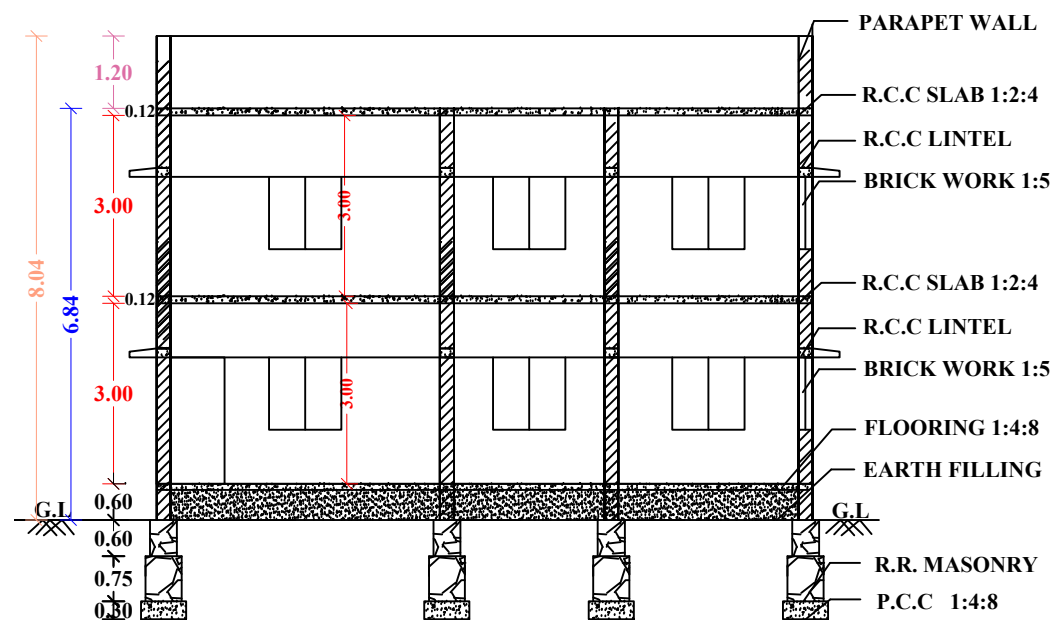
"SECTION "AB"
