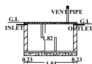
SEPTIC TANK DETAILS
