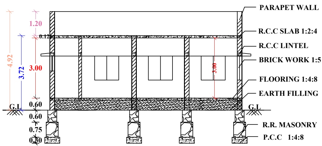
"SECTION "AB"
