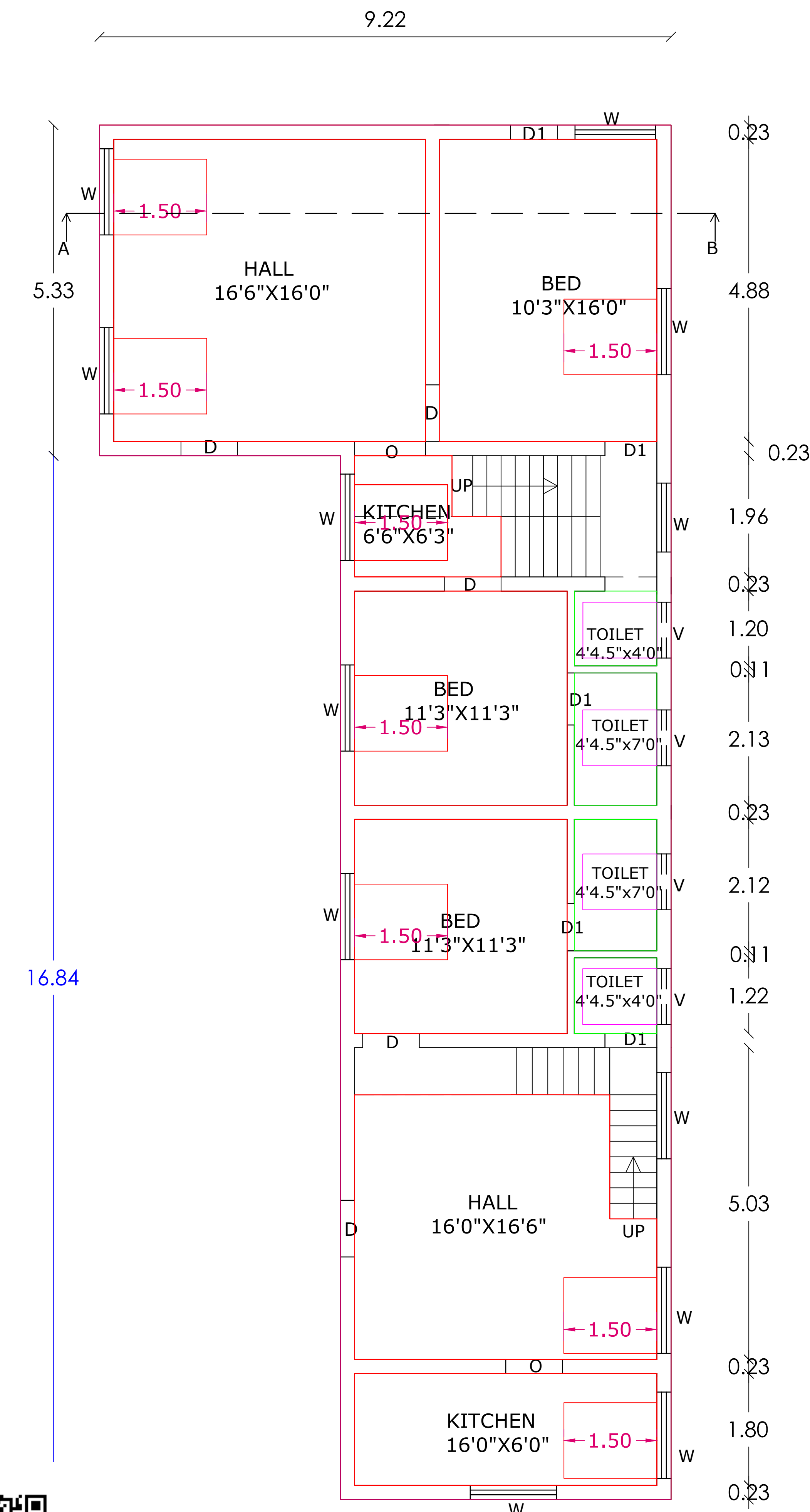
FLOOR PLAN
