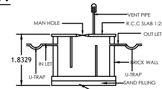
SECTION E-F SEPTIC TANK DETAIL
