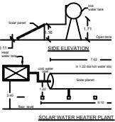
SOLAR WATER HEATER PLANT
