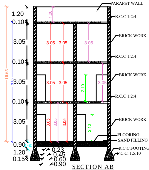
SECTION AB
