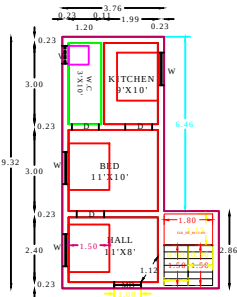
PRO FIRST FLOOR RESIDENTIAL PLAN
