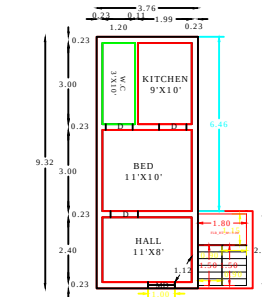
EXT GROUND FLOOR RESIDENTIAL PLAN
