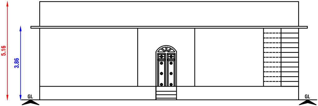
FRONT ELEVATION
