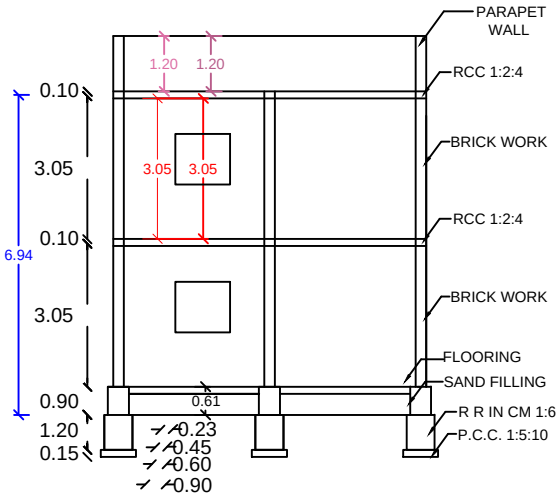
SECTION AB
