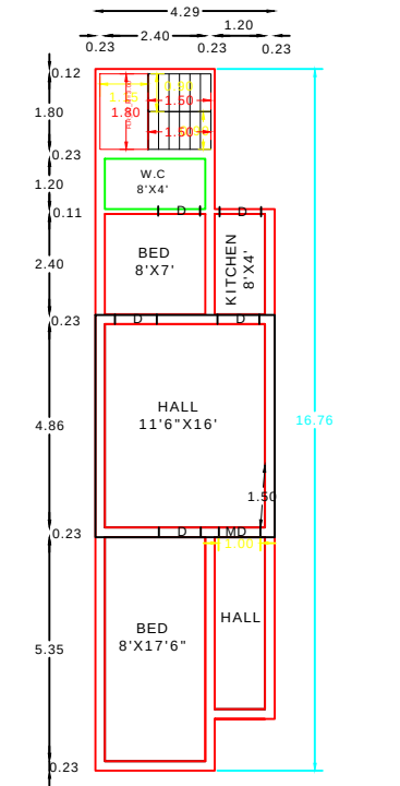
EXT GROUND FLOOR RESIDENTIAL PLAN
