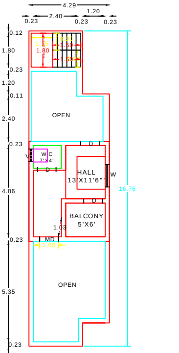
PRO FIRST FLOOR RESIDENTIAL PLAN
