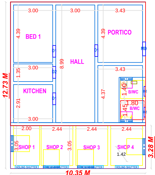
PLAN - GROUND FLOOR (PRO.BUILDING)
