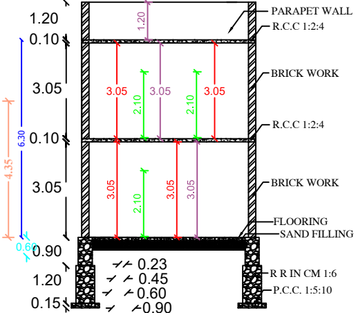
SECTION AB
