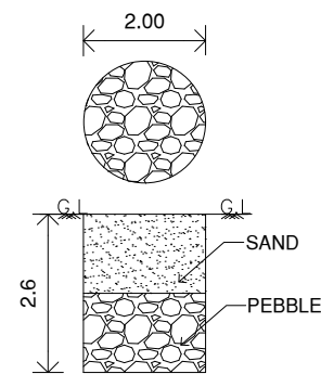
RAINWATER HARVESTING
