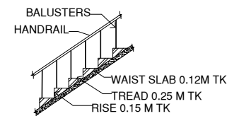
STAIRCASE DETAILS
