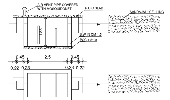
PLAN&SECTION OF SEPTIC TANK TRENCH
