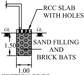
CROSS SECTION OF BS
