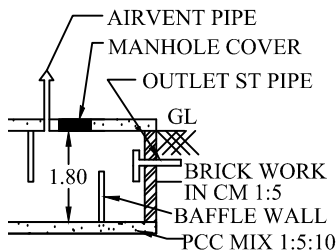
CROSS SECTION ON SEPTICTANK
