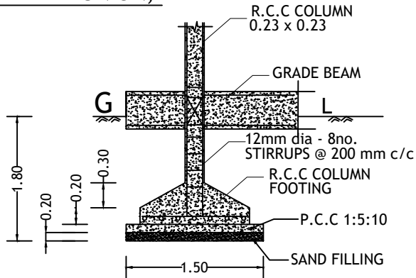
COLUMN - FOUNDATION DETAILS
