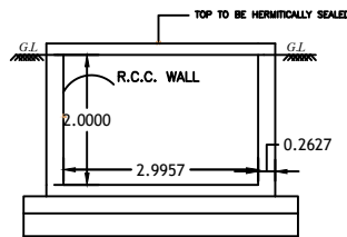
RWH SECTION
