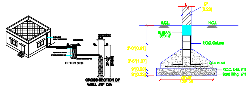
PRO.RAIN WATER SYSTEM
