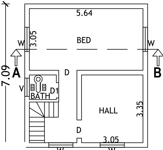
PLAN FIRST FLOOR (PROPOSED)
