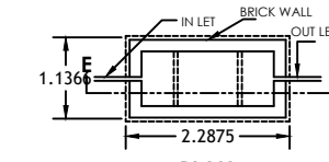
PLAN PLAN OF SEPTIC TANK
