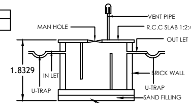
SECTION E-F SEPTIC TANK DETAIL
