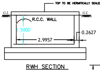
RWH SECTION
