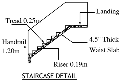
STAIRCASE DETAIL
