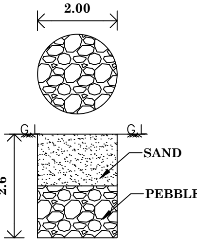
RAINWATER HARVESTING
