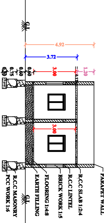
"SECTION "AB"
