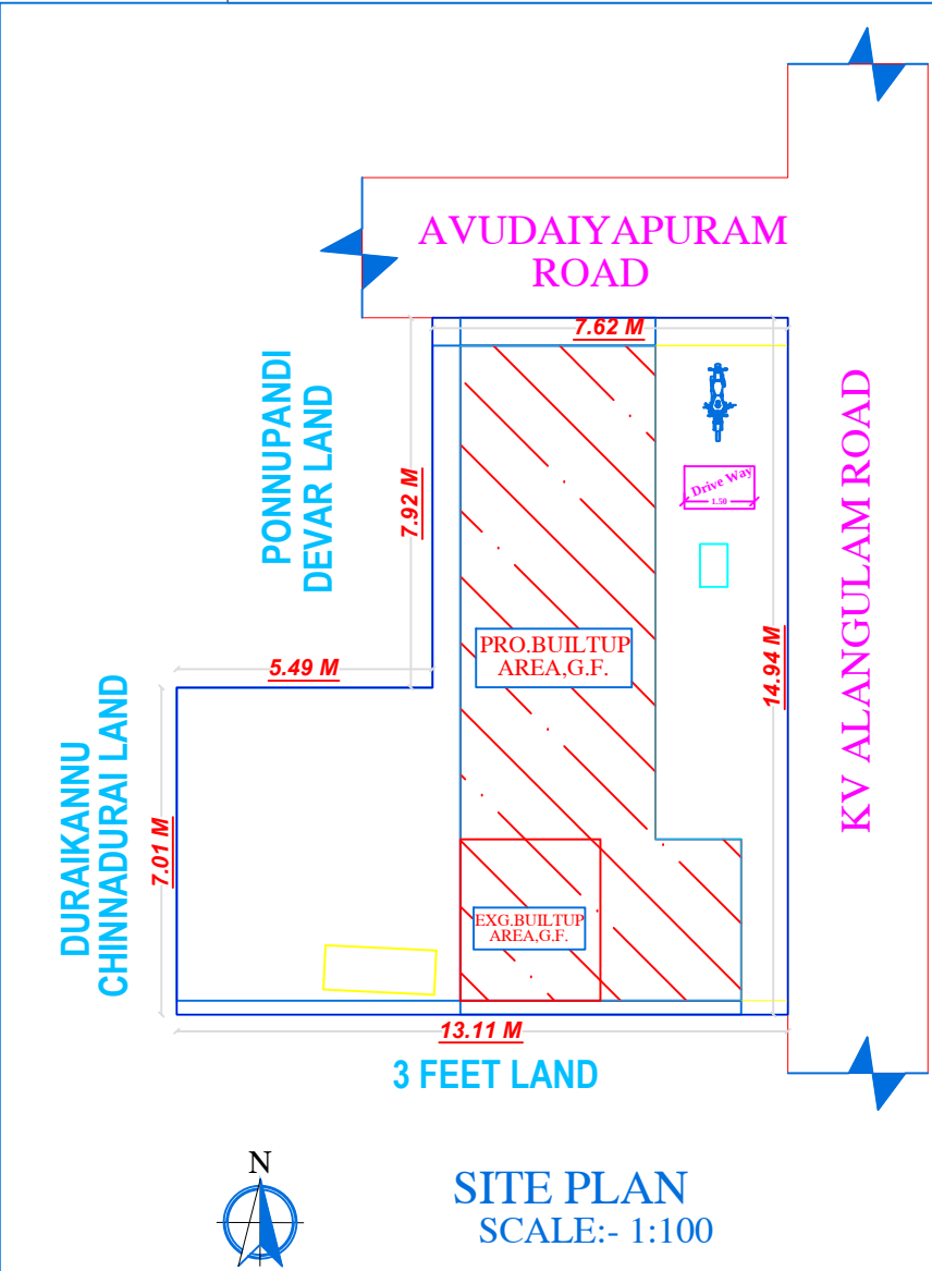
LOCATION PLAN
