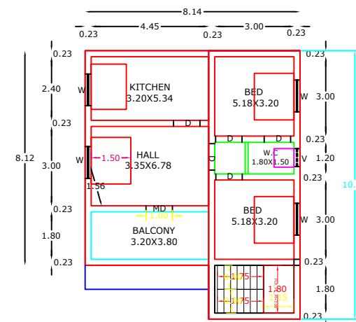
PRO FIRST FLOOR RESIDENTIAL PLAN
