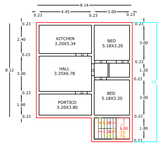
EXT GROUND FLOOR RESIDENTIAL PLAN
