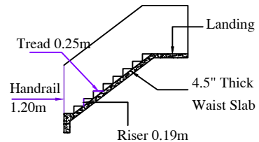
STAIRCASE DETAIL
