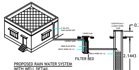
PROPOSED RAIN WATER SYSTEM WITH WELL DETAIL
