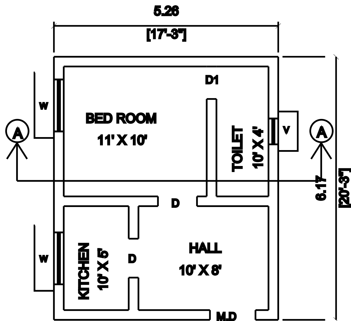
PLAN
